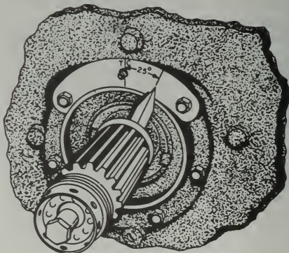
FIGURE 4-30. A timing plate and pointer
